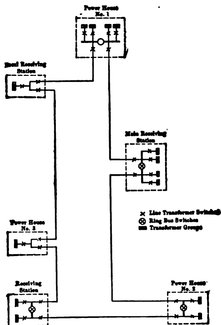
FIG. 3.—GENERAL ARRANGEMENT OF HIGH TENSION LINES AND SWITCHES FOR A NUMBER OF POWER HOUSES AND RECEIVING STATIONS, LAID OUT ON RING MAIN SYSTEM.
